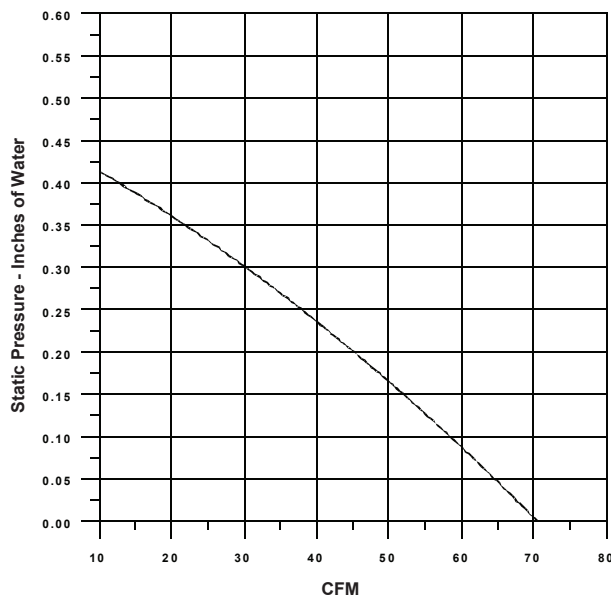
NuVent Product Performance Model NXSS50
